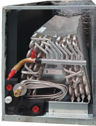
Unit shown with service panels removed. Representative photo only. Some models may vary in appearance. Duct opening dimensions can be ascertained by subtracting 1 1/2" for top opening width/depth, 3/4" for bottom opening.
